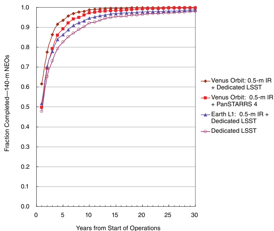
FIGURE 3.8 Years to 90 percent completion of the congressionally mandated survey for the detection of potentially hazardous near-Earth objects (NEOs) 140 meters in diameter or larger for combinations of space-based 0.5-meter infrared (IR) telescopes and ground-based telescopes. NOTE: LSST, Large Synoptic Survey Telescope; PanSTARRS, Panoramic Survey Telescope and Rapid Response System; L1, Lagrangian point 1. SOURCE: Courtesy of Steve Chesley, Jet Propulsion Laboratory.
